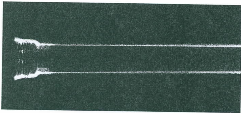
Fig. 25.10 Radiograph of an aluminum tubing with a crack.
