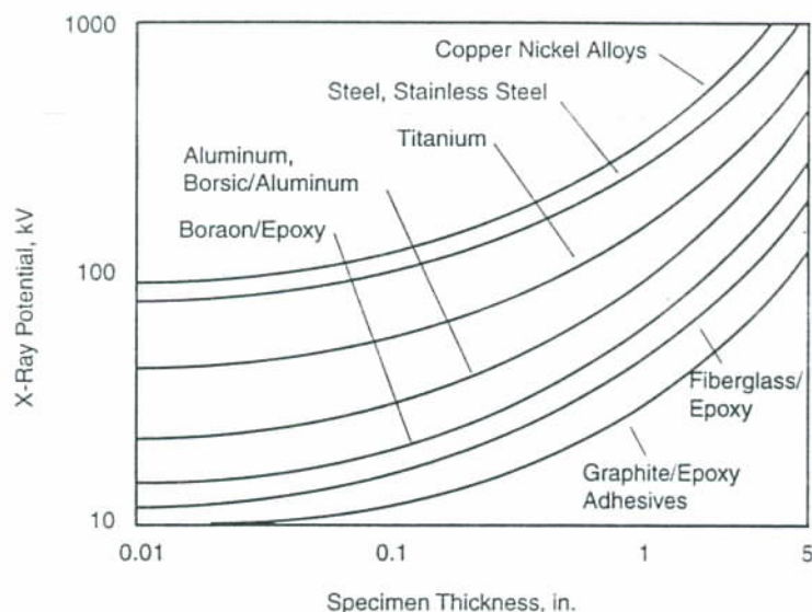
Fig. 25.11 Plot of the X-ray tube voltage vs. thickness for several important industrial materials.
