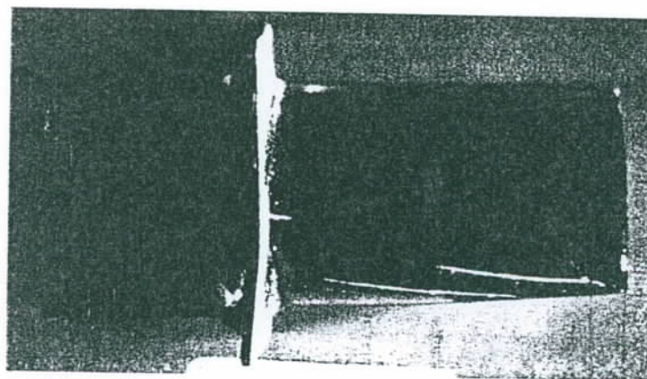
Fig. 25.2 Penetrant indication of a crack running along the edge of a jet engine turbine blade. Ultraviolet light causes the extracted penetrant to glow.
