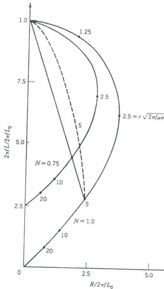
Fig. 25.21 The normalized impedance diagram for a long encircling coil on a solid, nonferromagnetic cylinder. For N = 1 the coil and cylinder have the same diameter; while for N = 0.75 the coil is approximately 1.155 times larger than the cylinder.
