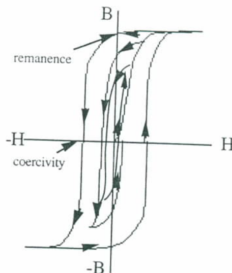
Fig. 25.26 A magnetic flux intensity, H , versus magnetic flux density, B , hysteresis curve for a typical steel. Initial magnetization starts at the origin and progresses as shown by the arrows. Demagnetization follows the arrows of the smaller hysteresis loops.
