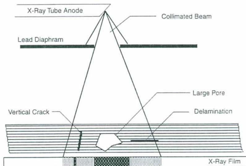
Fig. 25.9 Schematic radiograph of a thin plate with two types of flaws.
