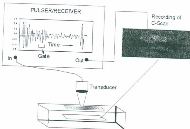
Fig. 25.7 Schematic representation of ultrasonic data collection. The data are displayed using the C-scan mode. The image shows a defect located at a certain depth in the material.
