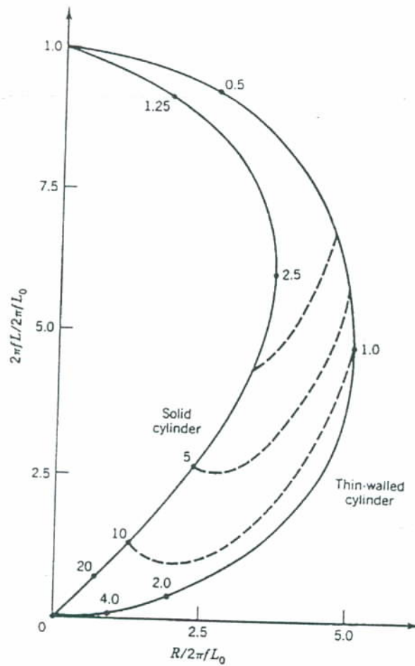
Fig. 25.22 The normalized impedance diagram for a long encircling coil on a solid and thin-walled solid, nonferromagnetic cylinders. The dashed lines represent the effects of varying wall thickness.
