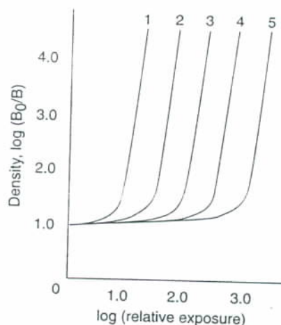
Fig. 25.15 Density vs. relative exposure for films that could be used in a multiple film exposure to obtain optimum flaw detectability in a complex part.
