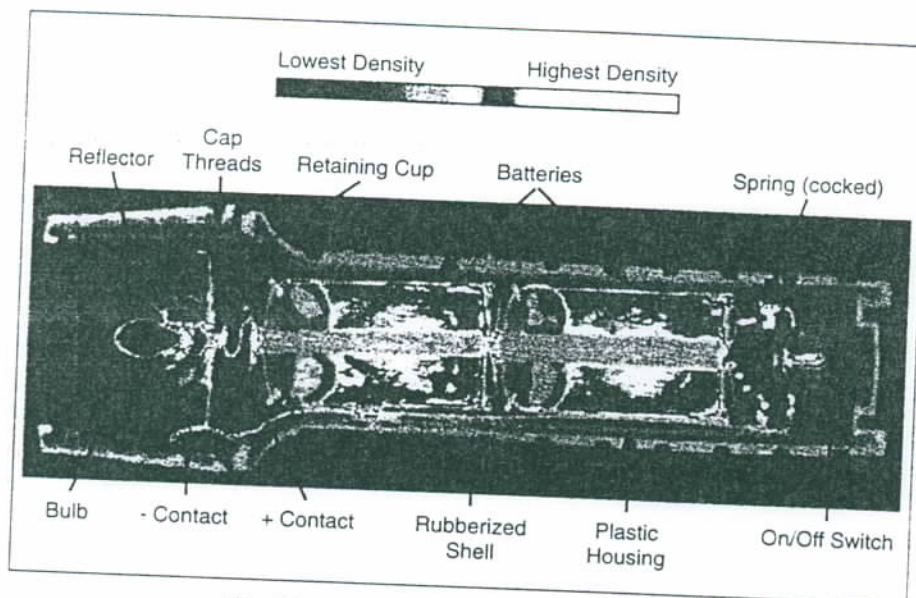
Fig. 25.18 Computed tomograph of flashlight.
