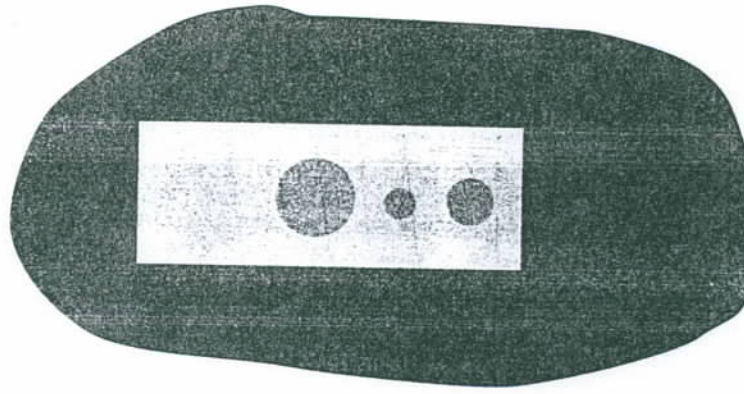
Fig. 25.17 Idealized radiograph of the penetrameter shown in Fig. 25.16. The 1T hole is just visible, indicating the resolution obtained in the radiograph.
