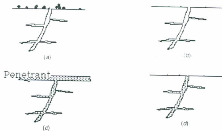
Fig. 25.1 (a) Schematic representation of a part surface before cleaning for penetrant inspection; (b) part surface after cleaning and before penetrant application; (c) part after penetrant application; (d) part after excess penetrant has been removed.
