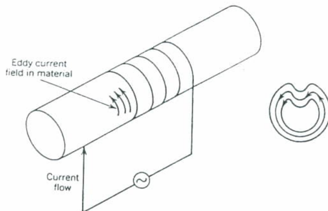
Fig. 25.20 Schematic representation of eddy current inspection of a solid cylinder. Also shown are the eddy current paths within the cross section of the cylinder in the vicinity of a crack.
