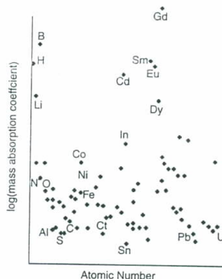
Fig. 25.12 A plot of neutron mass absorption coefficient vs. atomic number.
