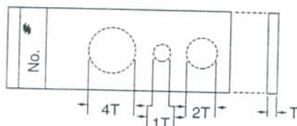
Fig. 25.16 Schematic of typical X-ray penetrameter.
