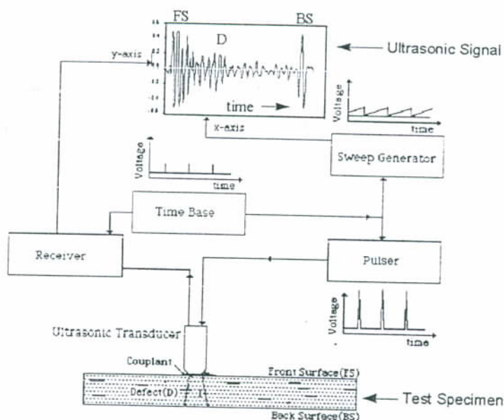
Fig. 25.3 Schematic representation of ultrasonic data collection and display in the A-scan mode.
