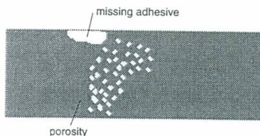
Fig. 25.13 Idealized neutron radiograph of bonded aluminum panel with two types of flaws.
