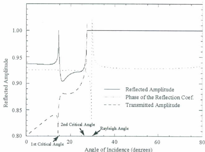
Fig. 25.6 Amplitude (energy flux) and phase of the reflected coefficient and transmitted amplitude vs. angle of incidence for a longitudinal wave incident on a water-steel interface. The arrows indicate the critical angles for the interface.
