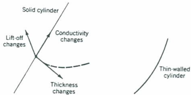
Fig. 25.23 The effects of various changes in inspection conditions on signal changes in the impedance plane of Fig. 25.22. Phase differentiation is relatively easily accomplished with current instrumentation.
