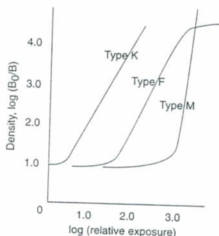
Fig. 25.14 Density or darkness of X-ray film vs. relative exposure for three common radiography films.
